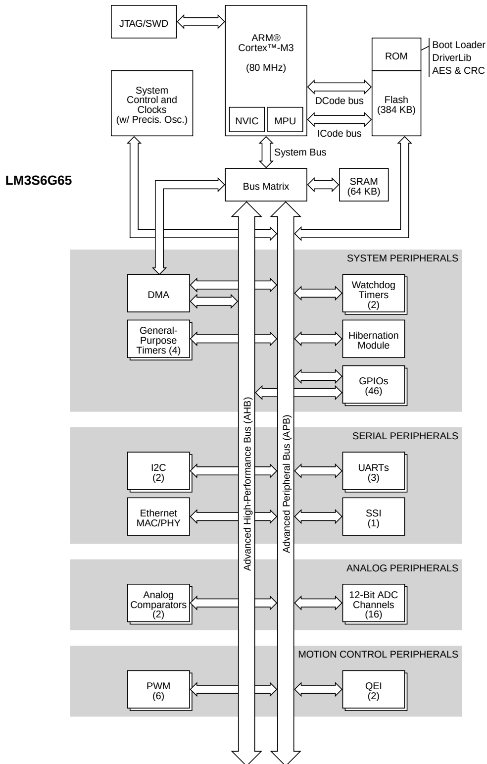
Figure 1-1. Stellaris LM3S6G65 Microcontroller High-Level Block Diagram
